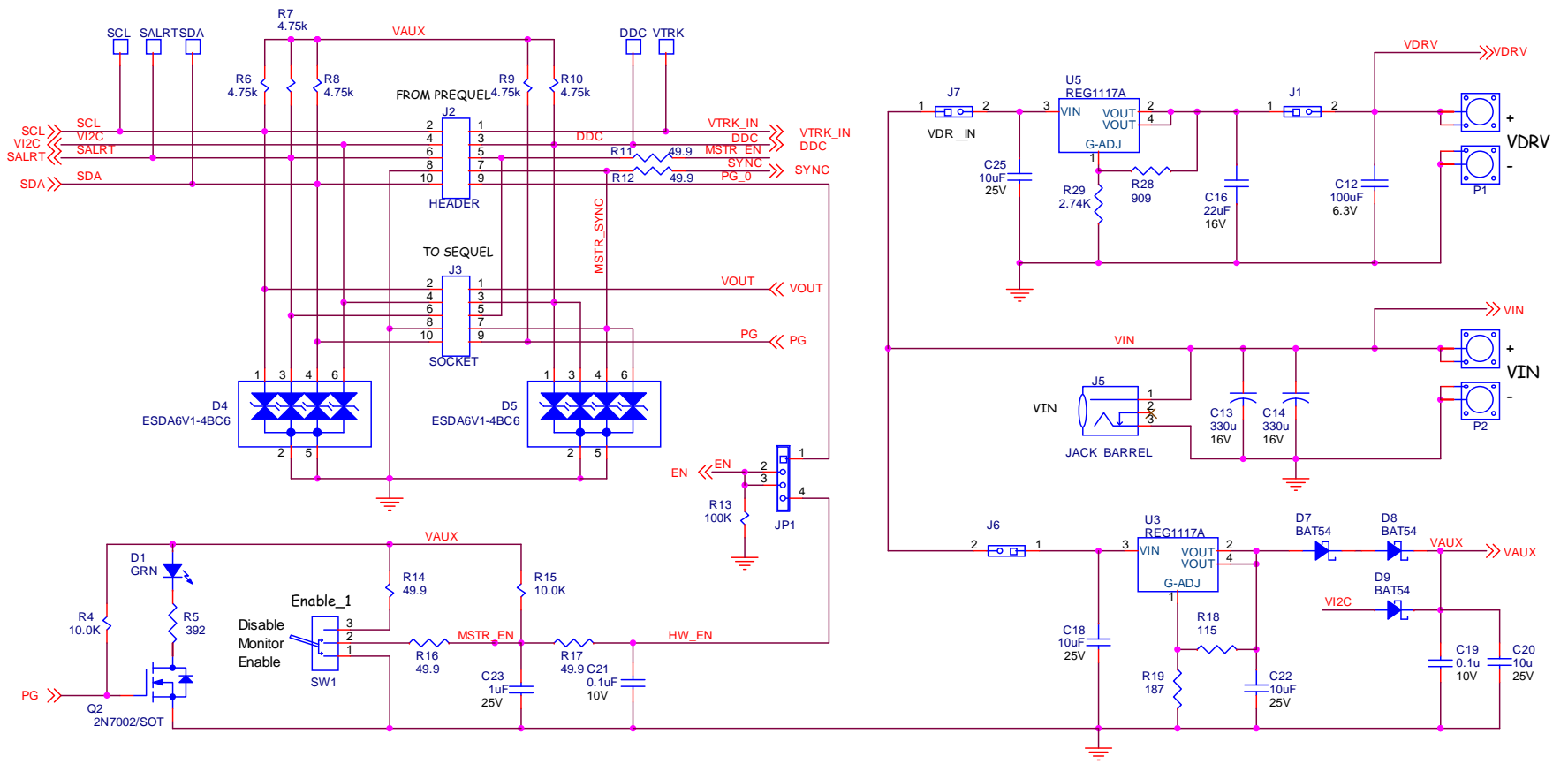
FIGURE 3. ZL8101_30AEV2Z 30A DEMO BOARD – INTERFACE CIRCUITRY
